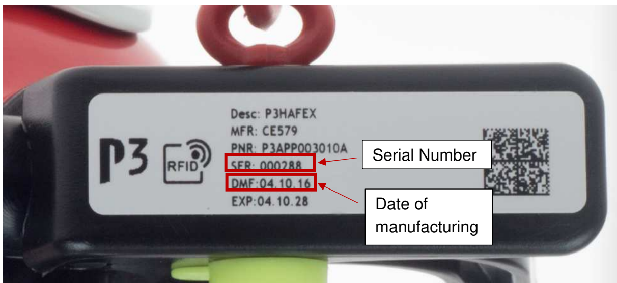
Figure 1: RFID Label.
